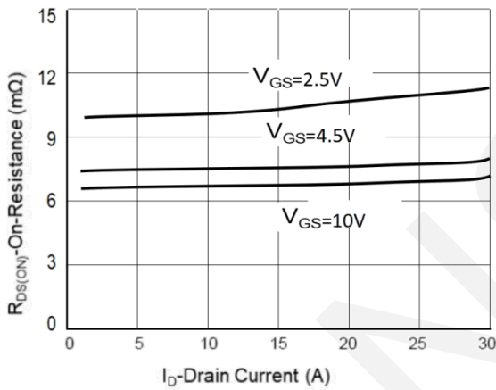
Rdson-Drain Current
