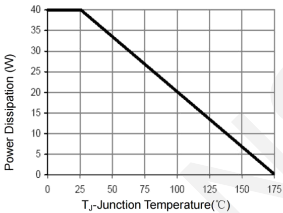
Power De-rating
