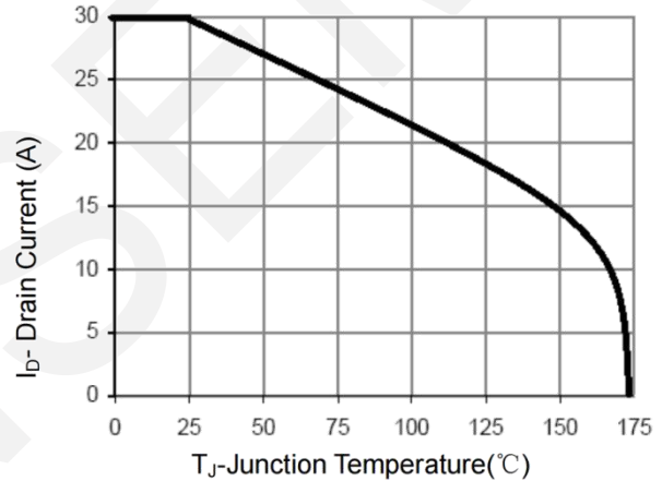
ID Current Derating
