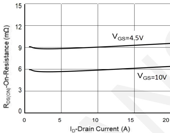
Rdson-Drain Current
