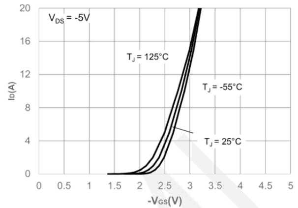
Transfer Characteristics
