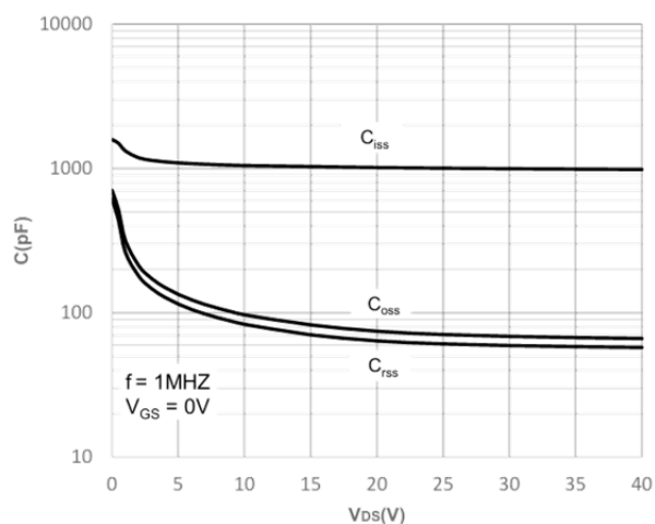
Capacitance Characteristics
