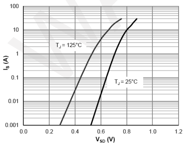
Body-diode Characteristics
