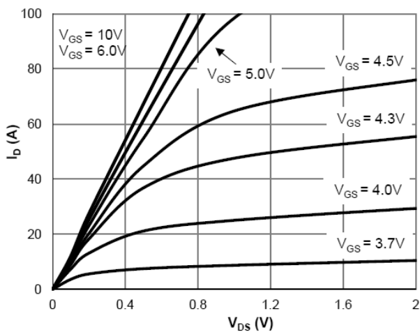
Saturation Characteristics
