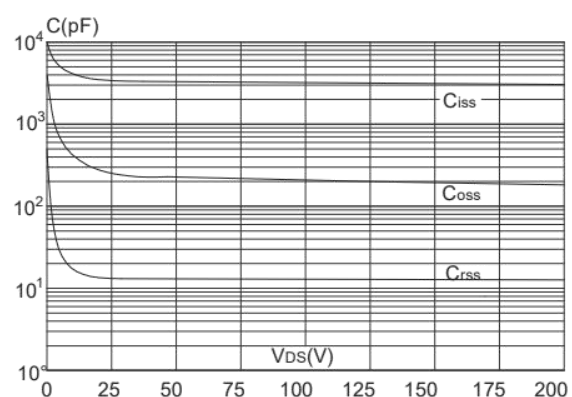
Capacitance Characteristics
