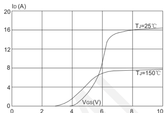
Transfer Characteristics
