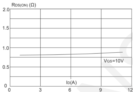
Rdson-Drain Current
