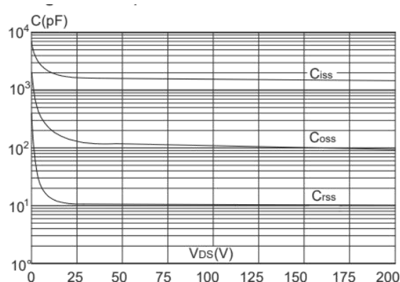
Capacitance Characteristics
