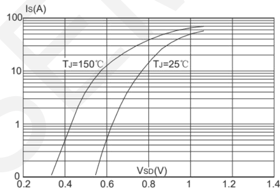
Body Diode Characteristic
