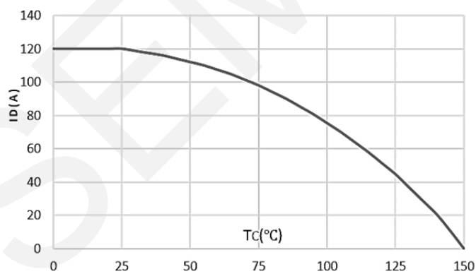
Maximum Continuous Drain Current vs. Case Temperature
