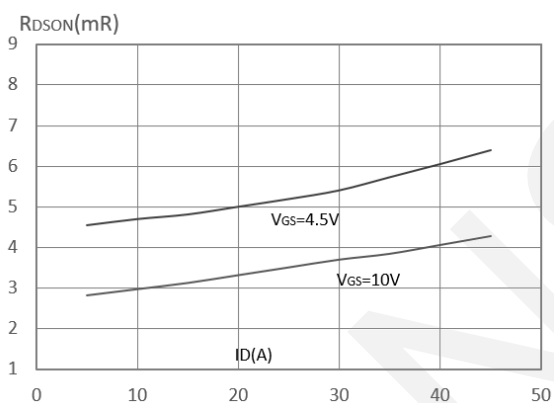
Rdson-Drain Current
