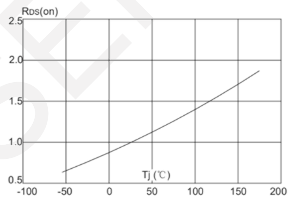
Rdson-Junction Temperature
