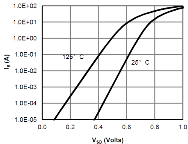
Body-Diode Characteristics
