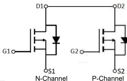
Schematic Diagram
