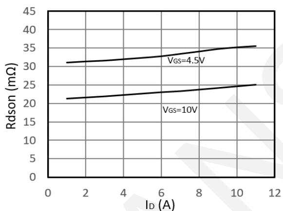
Drain-Source On-Resistance
