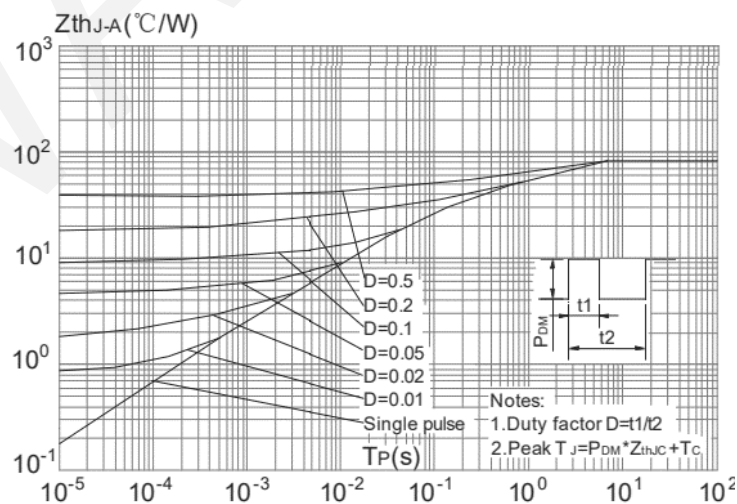
Maximum Effective Transient Thermal Impedance, Junction-to-Case
