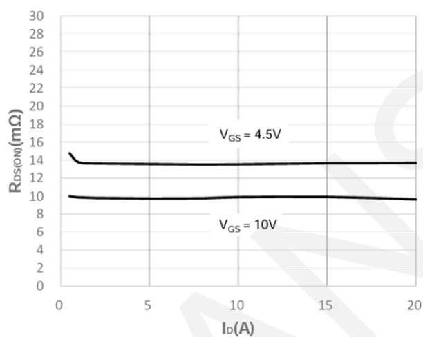
Rdson-Drain Current
