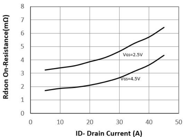
Rdson-Drain Current
