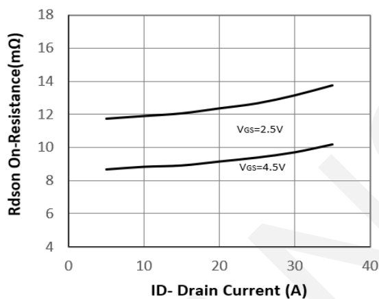
Rdson-Drain Current
