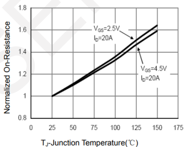
Rdson-Junction Temperature
