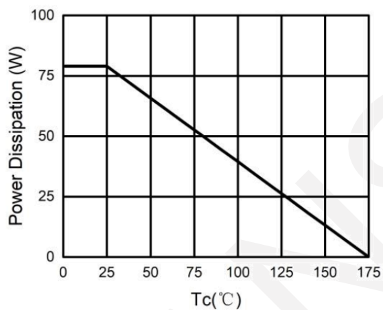
Power De-rating
