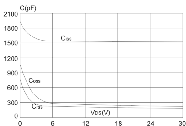
Capacitance Characteristics
