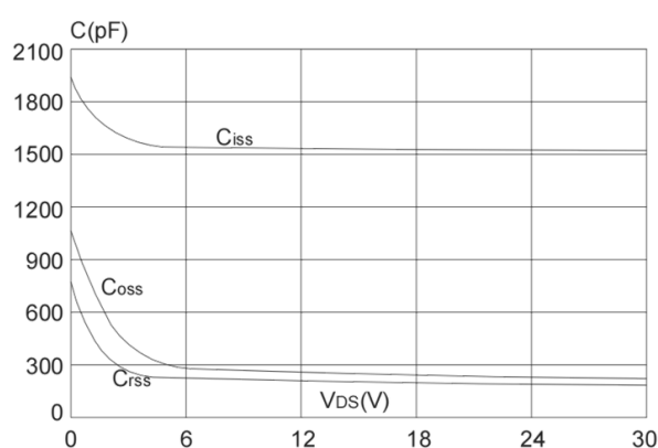
Capacitance Characteristics
