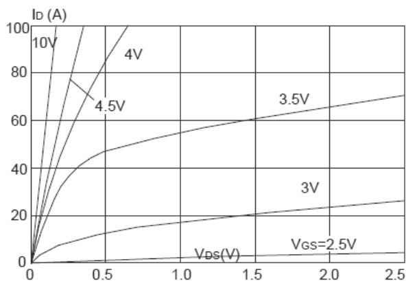
Output Characteristics
