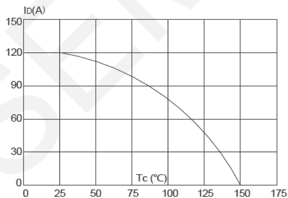
Continuous Drain Current vs. Case Temperature
