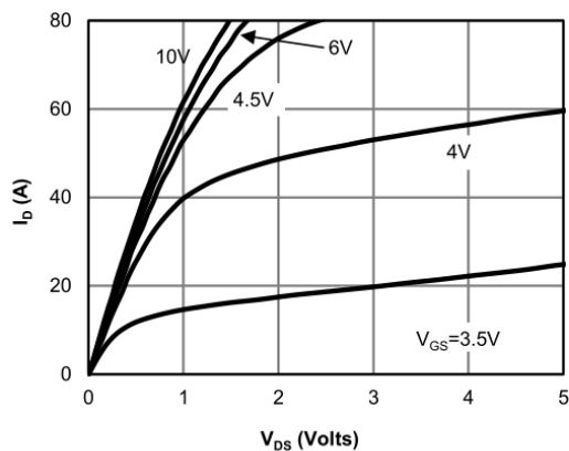
Output Characteristics
