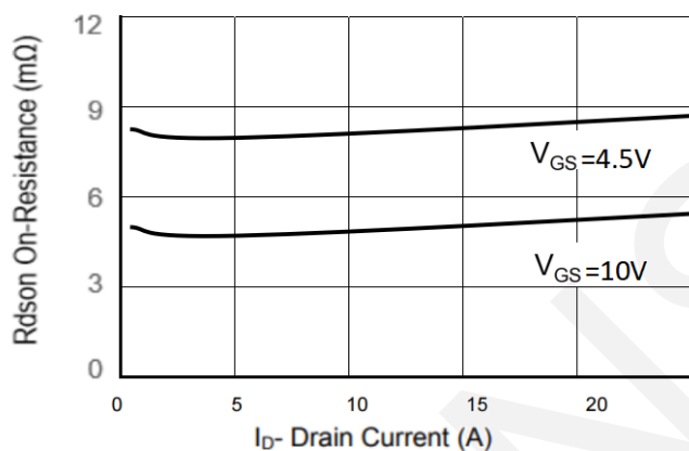
Rdson-Drain Current
