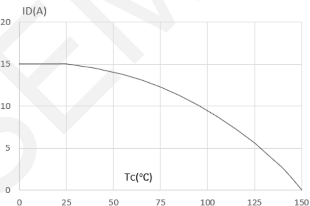
Maximum Continuous Drain Current - Case Temperature
