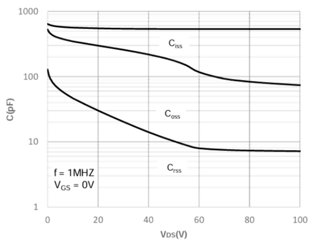
Capacitance Characteristics
