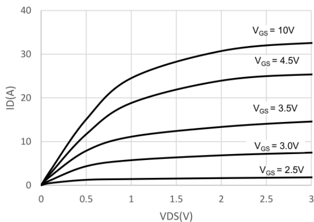
Output Characteristics
