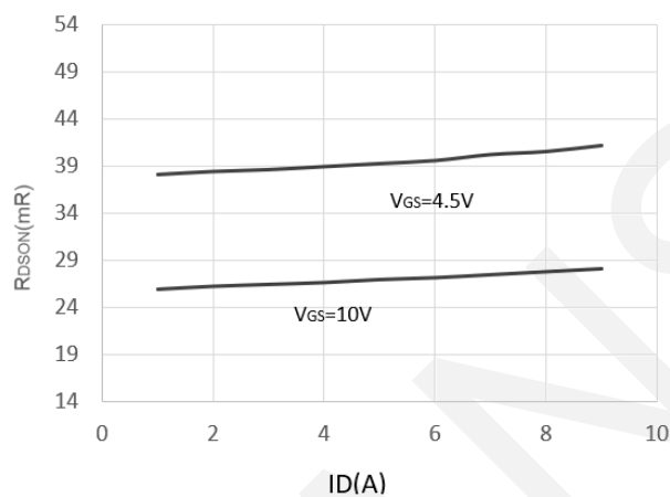
Drain-Source On-Resistance
