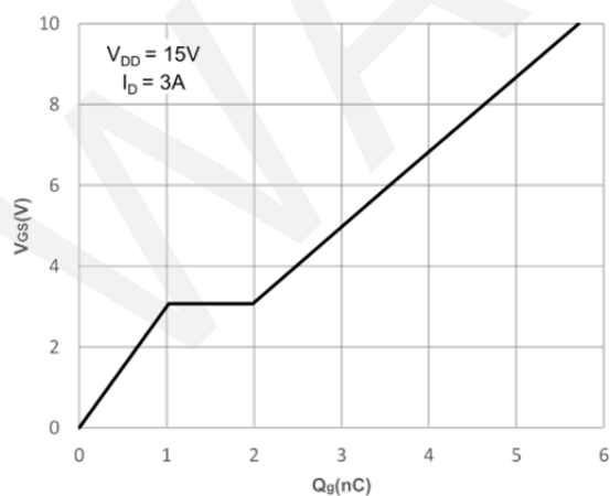
Gate Charge Characteristic
