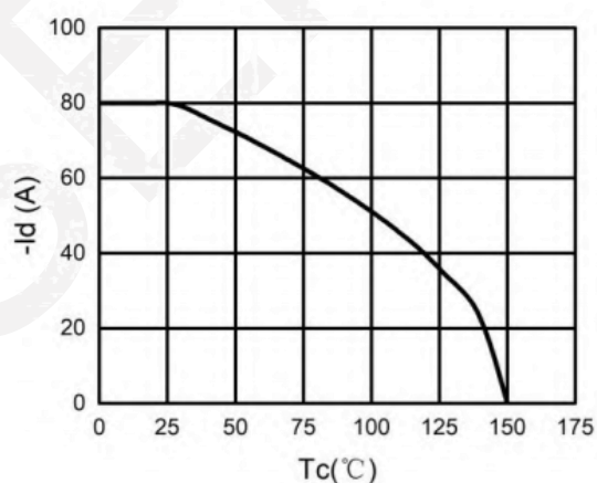
Drain Current
