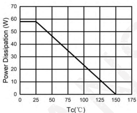
Power Dissipation
