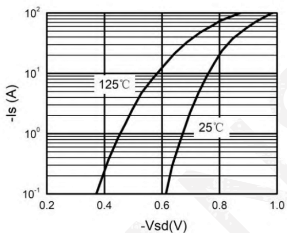
Body-Diode Characteristics
