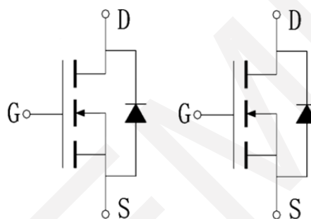
Schematic Diagram
