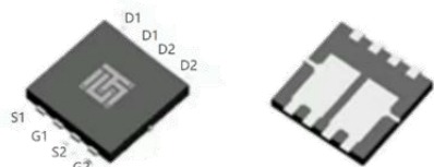
PDFN3X3 Pin Description
