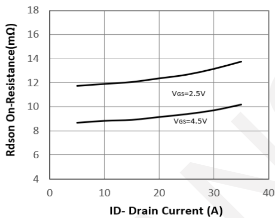
Rdson-Drain Current
