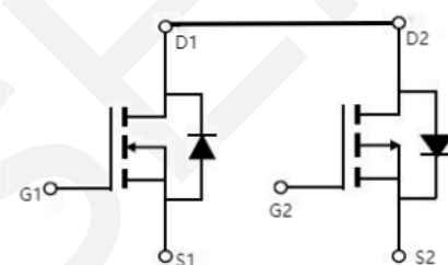
N-Channel
