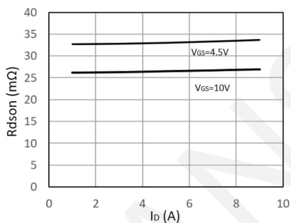
Drain-Source On-Resistance
