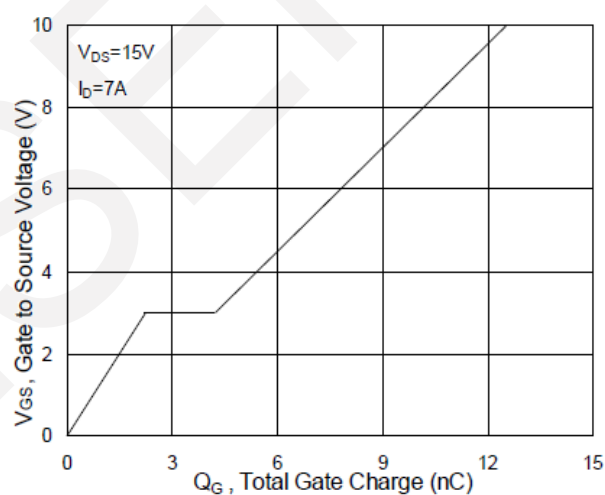
Gate-Charge Characteristics
