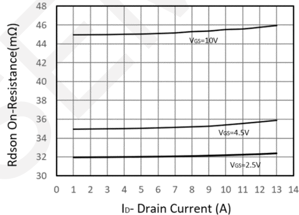
Drain-Source On-Resistance
