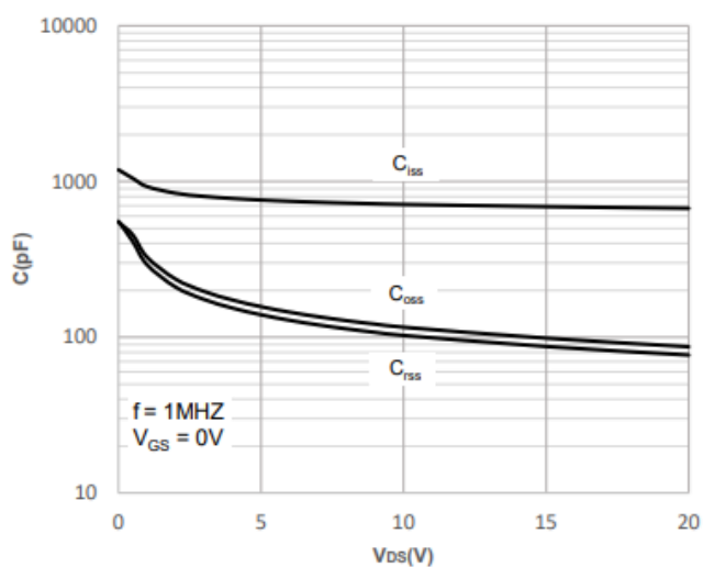
Capacitance Characteristics
