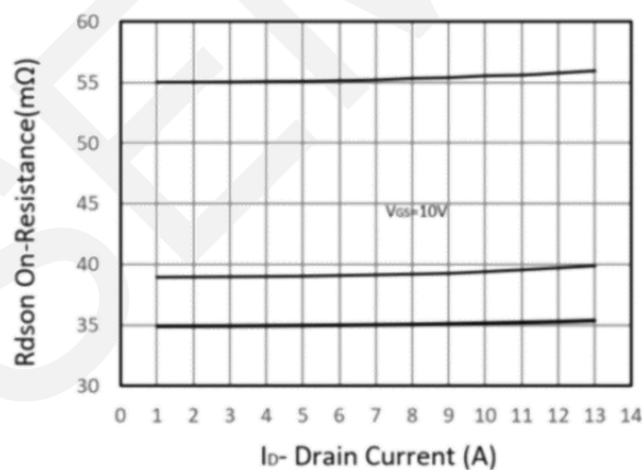
Drain-Source On-Resistance
