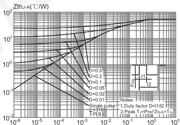
Maximum Effective Transient Thermal Impedance, Junction-to-Ambient
