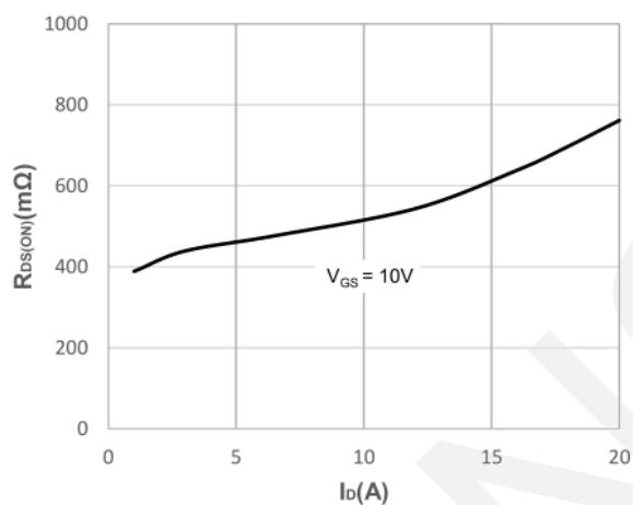
Rdson-Drain Current
