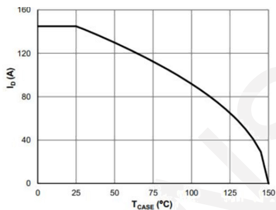
Current De-rating
