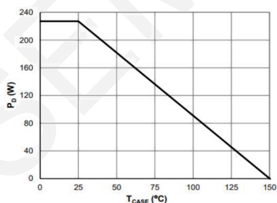
Power De-rating
