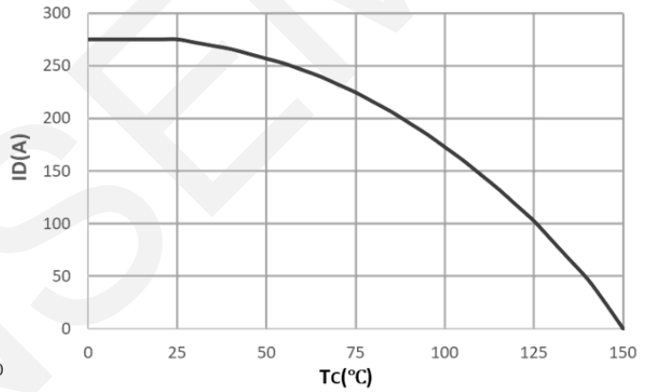
Maximum Continuous Drain Current vs. Case Temperature
