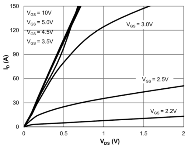
Saturation Characteristics
