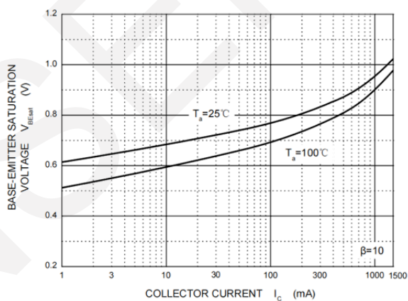
V_{EBsat} \sim I_C
