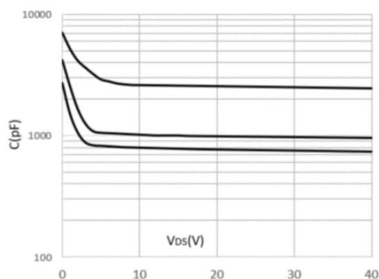
Capacitance Characteristics
