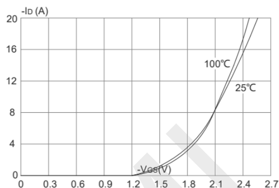
Transfer Characteristics
