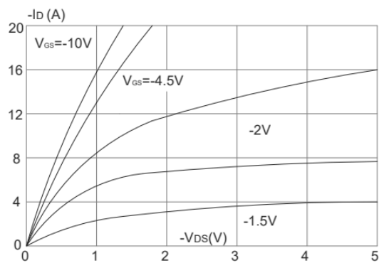
Output Characteristics
