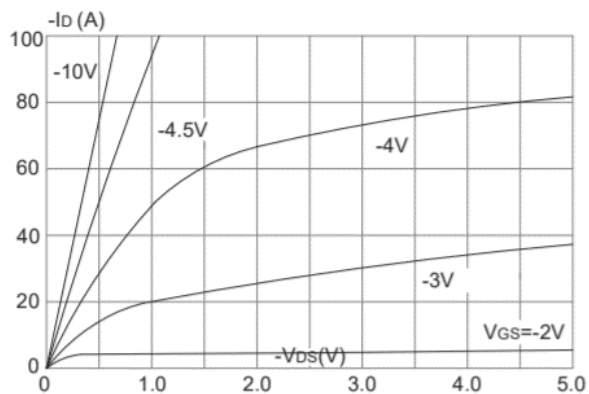
Output Characteristics
