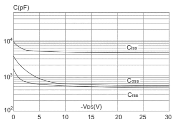
Capacitance Characteristics
