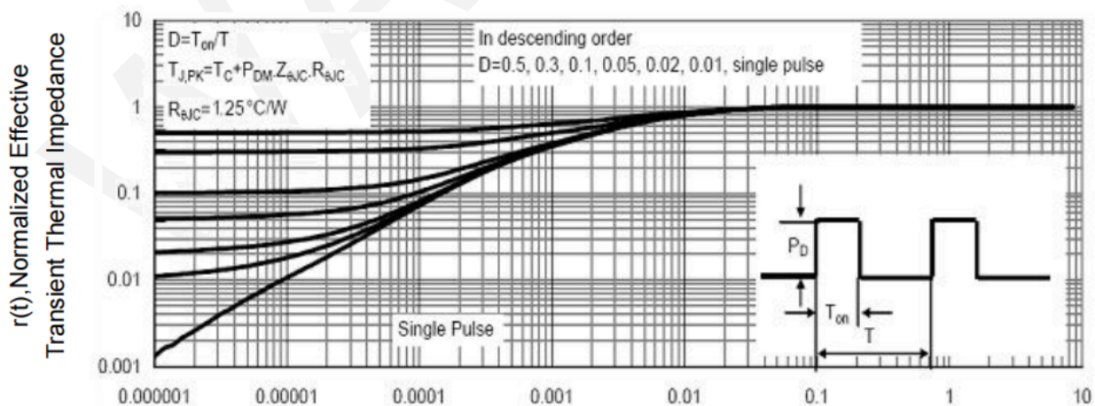
Square Wave Pulse Duration(sec) Maximum Effective Transient Thermal Impedance, Junction-to-Case
