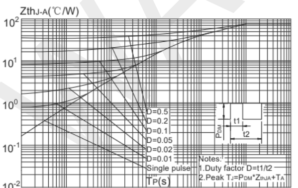
Maximum Effective Transient Thermal Impedance, Junction-to-Ambient
