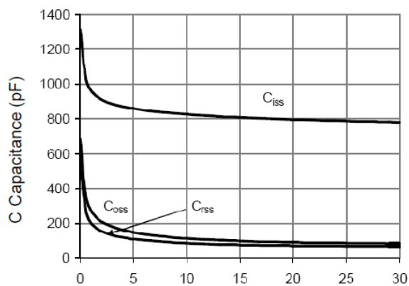
Capacitance Characteristics
