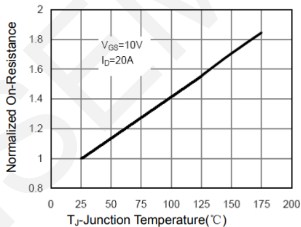
Rdson-Junction Temperature
