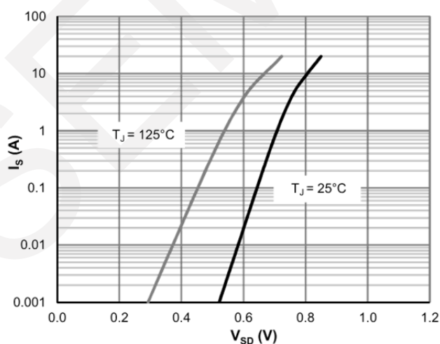
Body-Diode Characteristics
