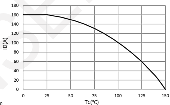
Current De-rating
