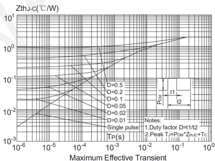
Thermal Impedance, Junction-to-Case
