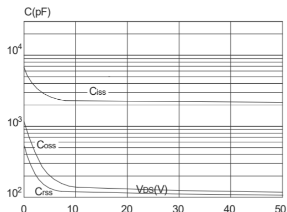
Capacitance Characteristics
