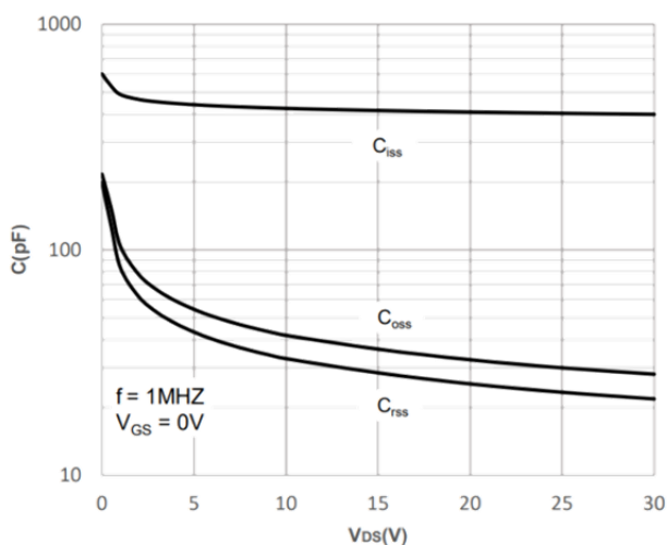
Capacitance Characteristics
