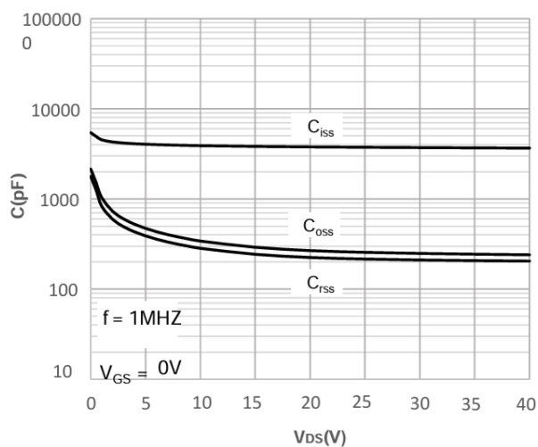
Capacitance Characteristics
