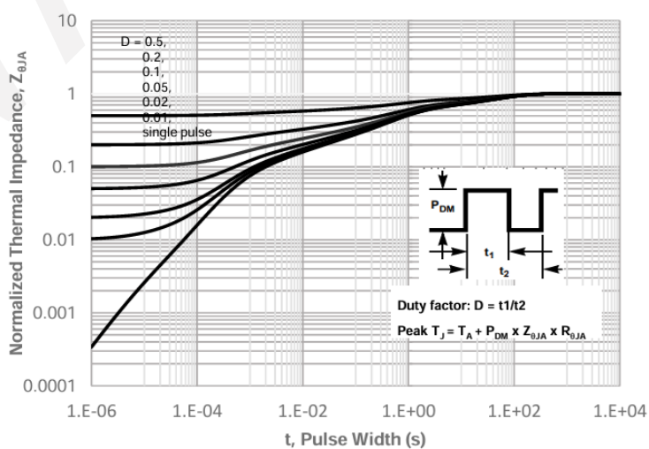
Figure 11 Maximum Transient Thermal Impedance WAN SEMICONDUCTOR (NINGBO) CO.,LTD
