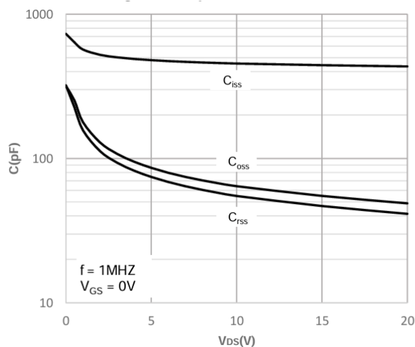
Figure 6 Capacitance Characteristics
