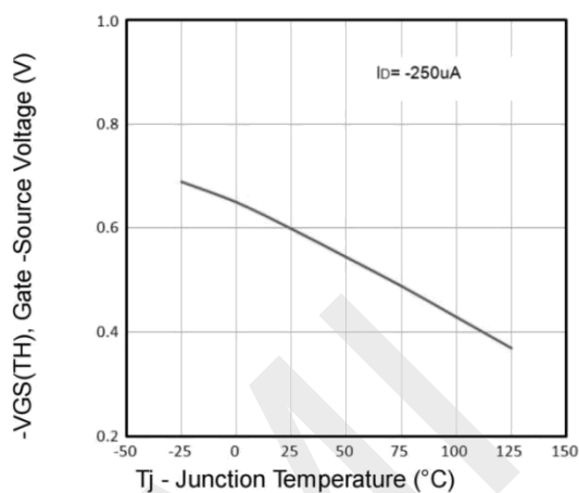
Normalized Threshold Voltage Vs. Temperature
